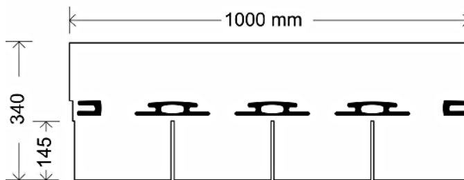
Fig. 1 - Rectangular shingle dimensions
