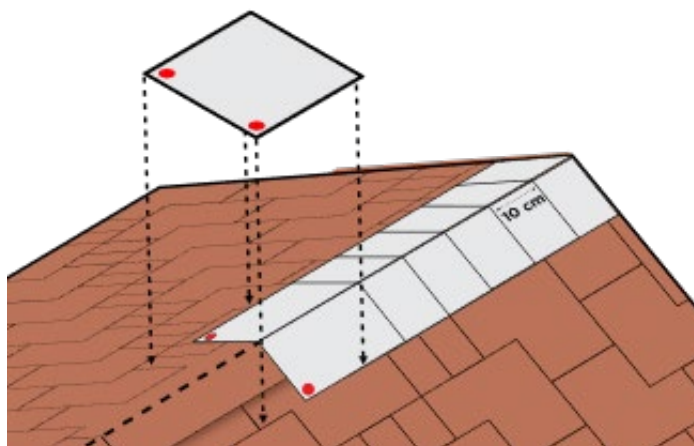
Fig. 11 - Ridge elements installation
