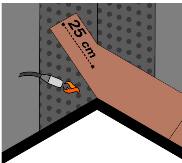
Fig. 20 - Shingles installation by torch at the valley
