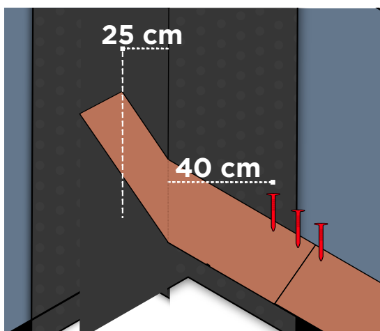
Fig. 12 - Shingles installation at valleys
