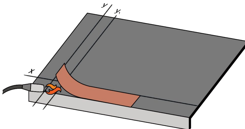
Fig. 16 - Starting row shingles installation by torch
