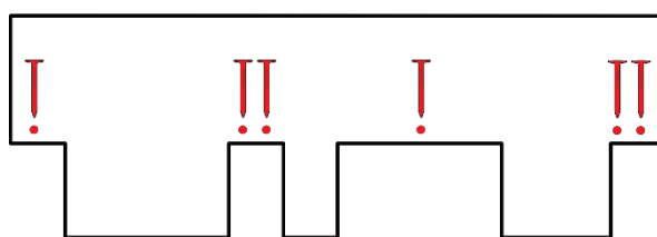
Fig. 8 - Shingle nailing a) slopes <60°; b) slopes >60°
