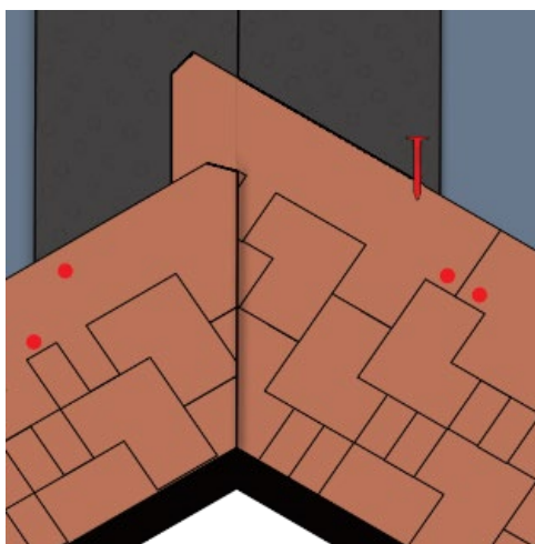
Fig. 13 - Shingles installation at valleys
