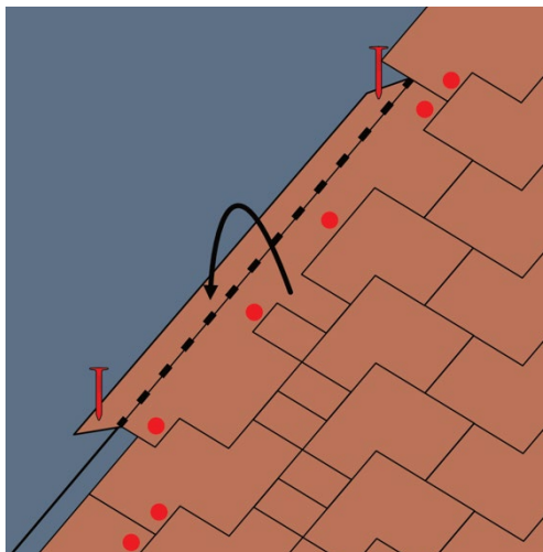
Fig. 9 - Shingles installation at the ridge
