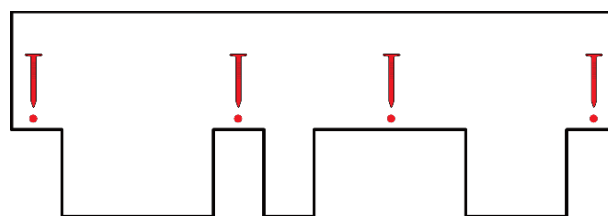
Fig. 7 - Shingles installation
