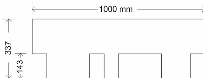
Fig. 1 - Gothic shingle dimensions
