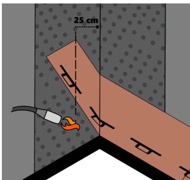
Fig. 20 - Shingles installation by torch at the valley
