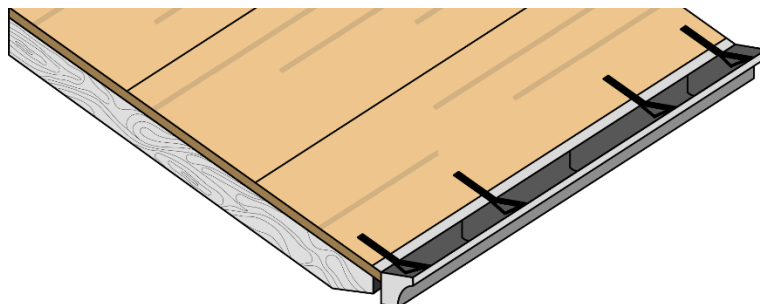
Fig. 2 - Gutter installation
