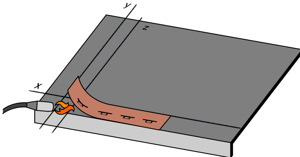
Fig. 16 - Starting row shingles installation by torch
