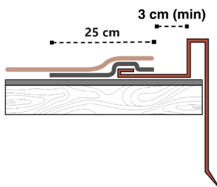
Fig. 15 - Lateral flashing detail
