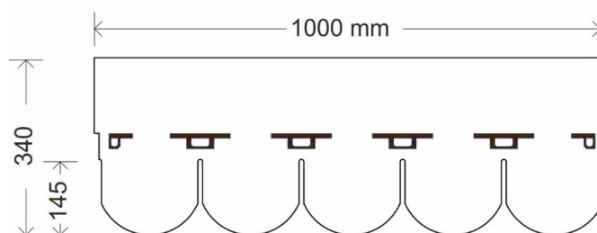
Fig. 1 - Traditional shingle dimensions
