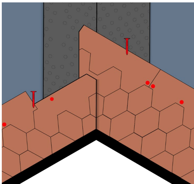
Fig. 13 - Shingles installation at valleys
