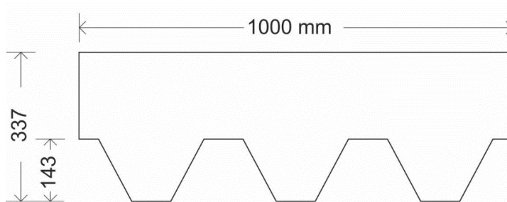
Fig. 1 - Mosaik shingle dimensions
