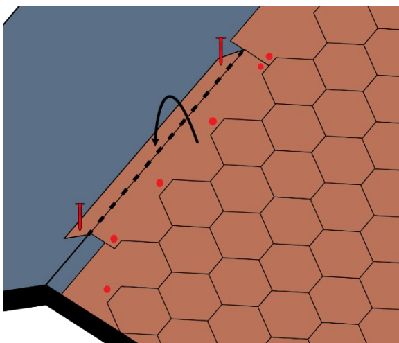
Fig. 9 - Shingles installation at the ridge
