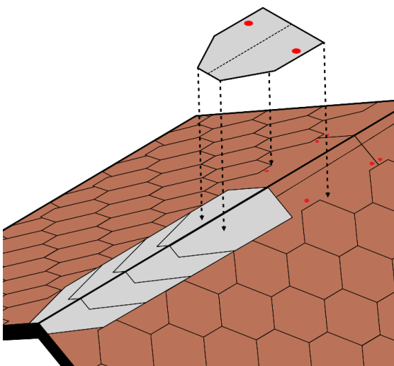
Fig. 11 - Ridge elements installation
